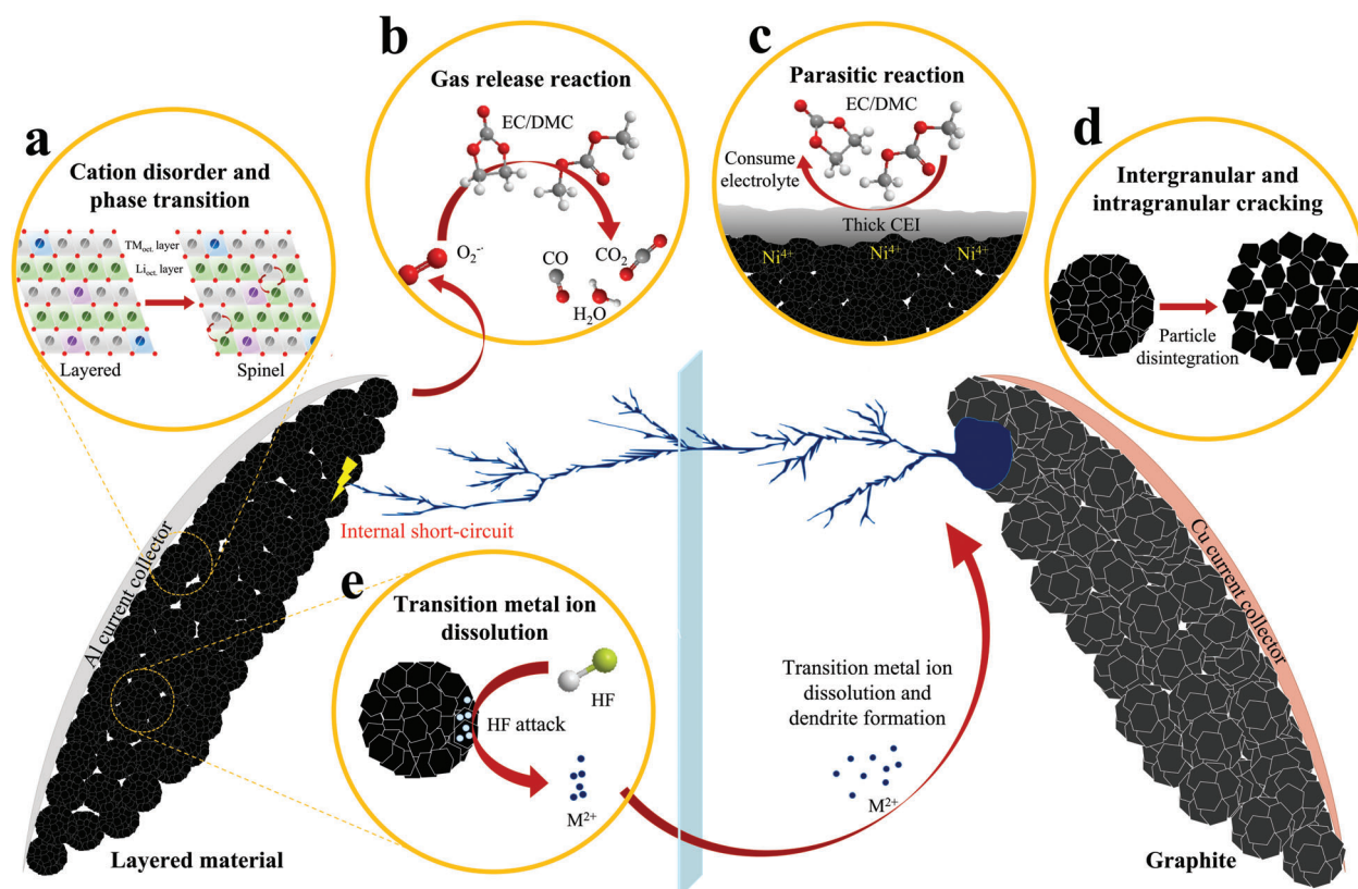
Figure 2. Schematic representation of the key challenges of layered cathodes in LIBs: a) cation disorder and phase transition, b) gas release reaction, c) parasitic reaction, d) intergranular and intragranular cracking, and e) transition metal ion dissolution.
